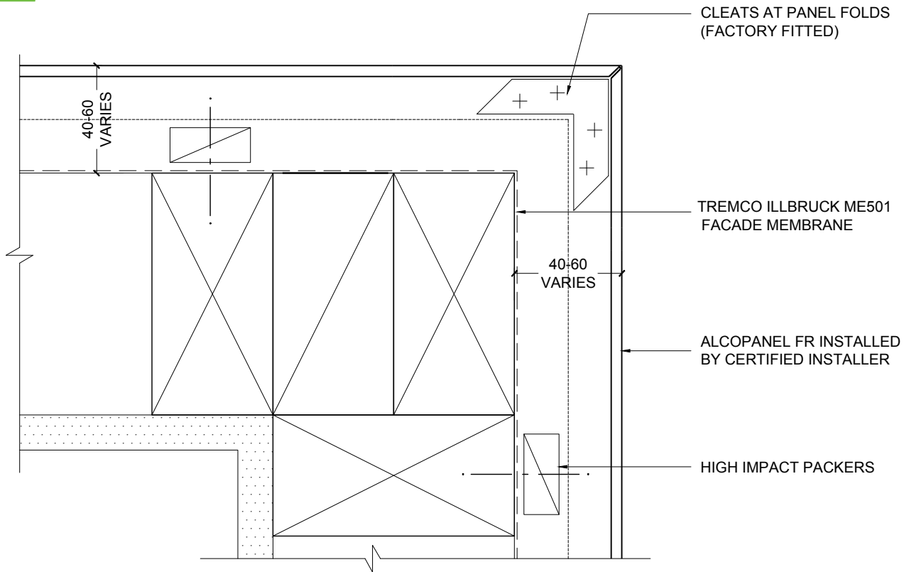
1 TYPICAL CORNER 1:2 @ A4
