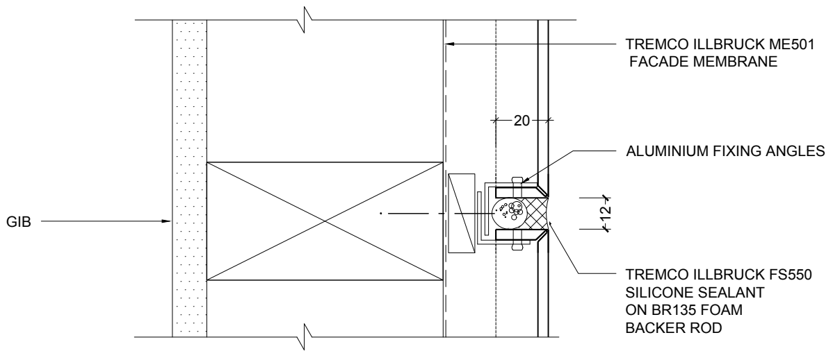
2 TYPICAL VERTICAL JOINT 1:2 @ A4
