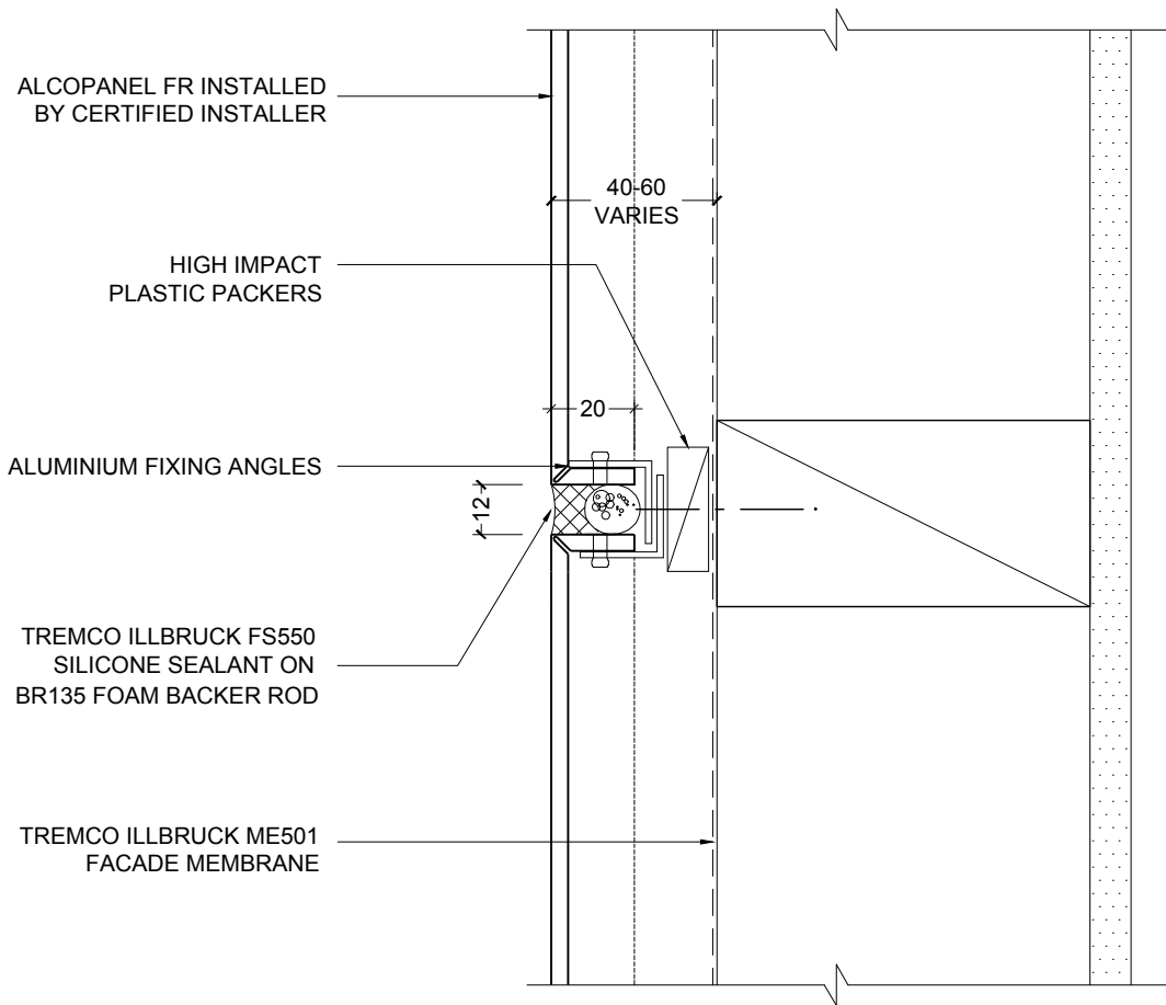
1 TYPICAL HORIZONTAL JOINT - 1:2 @ A4
