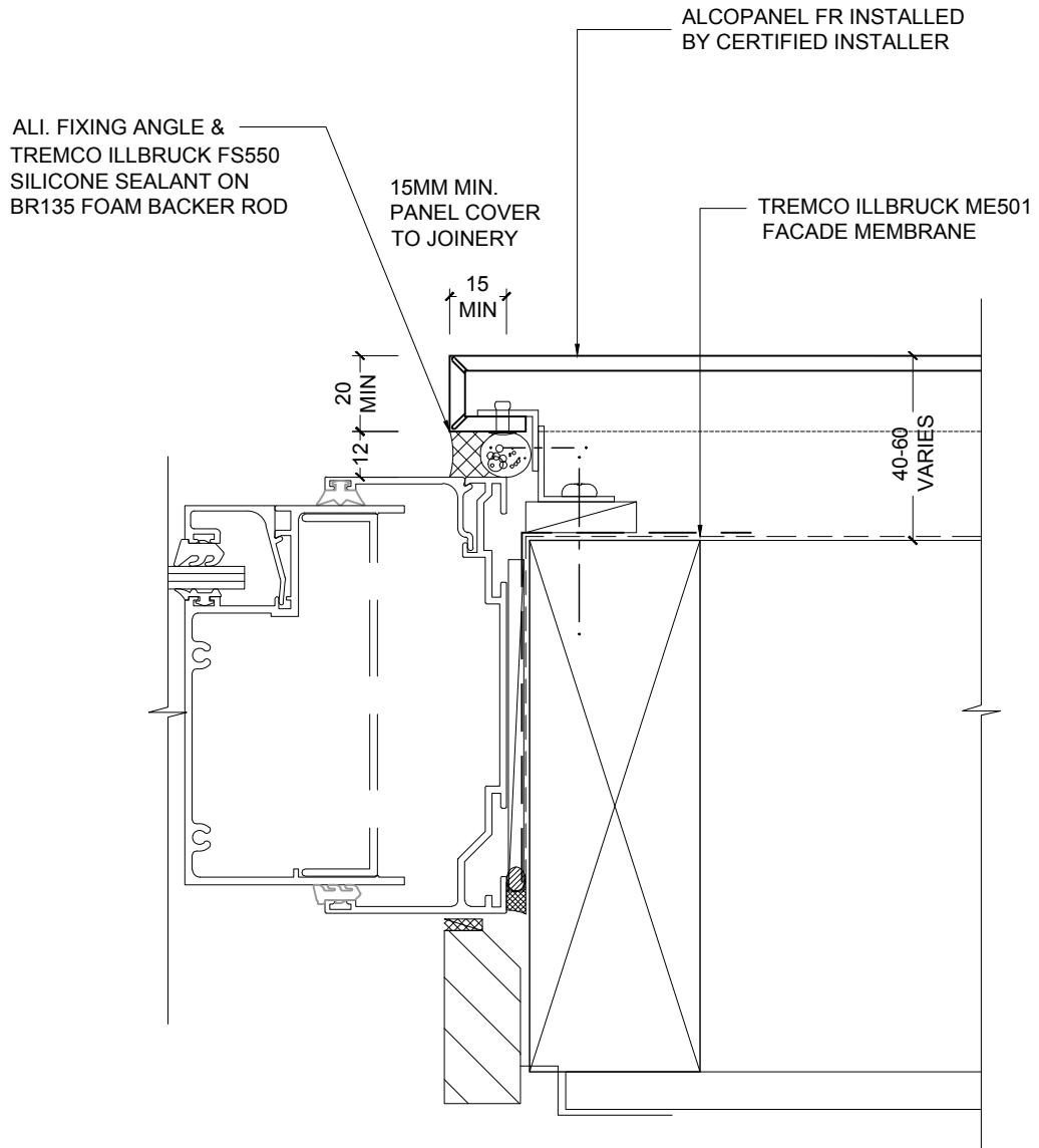
1 TYPICAL COMMERCIAL JAMB DETAIL - 1:2 @ A4
